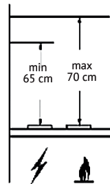
E-Herd Gasherd
